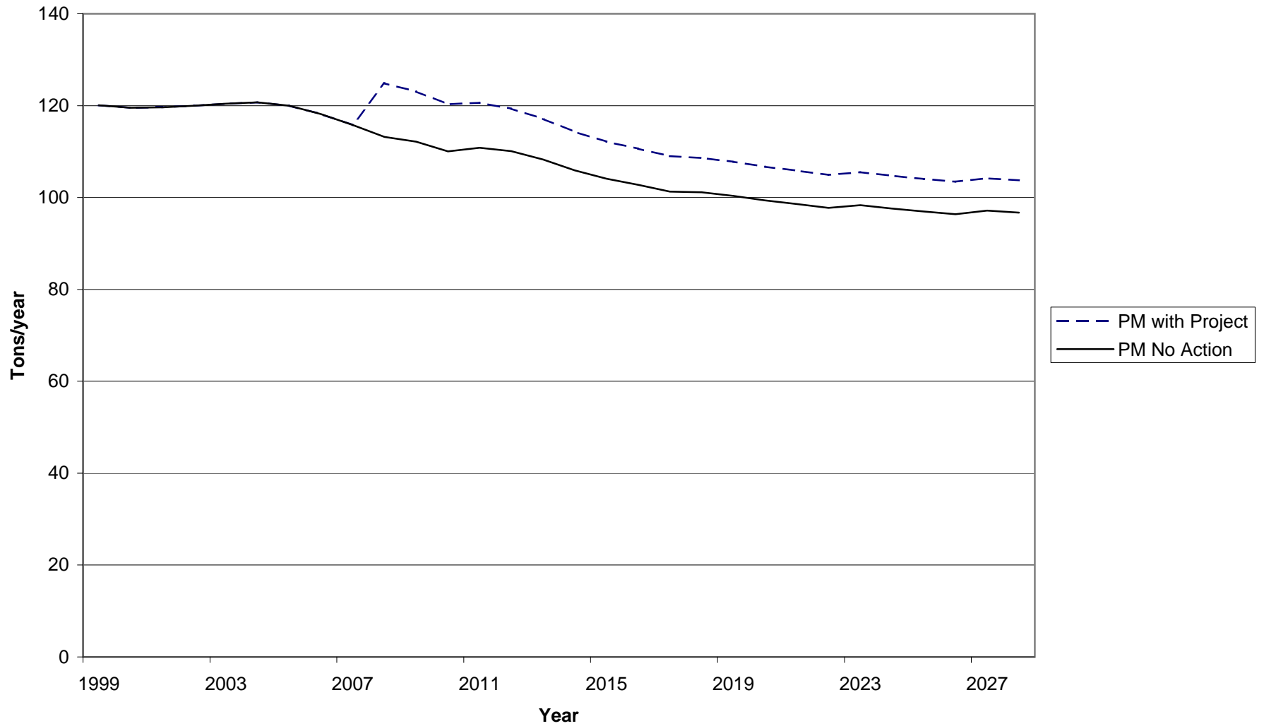
Figure K-3. Particulate Matter (PM) Emission Projections for Cascade Locks Resort and Casino and No Action Alternative
