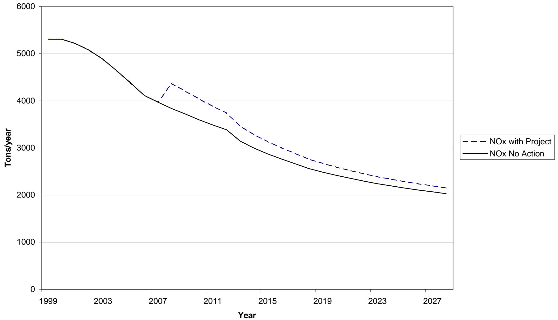
Figure K-4. Nitrogen Oxides (NO x ) Emission Projections for Cascade Locks Resort and Casino and No Action Alternative
