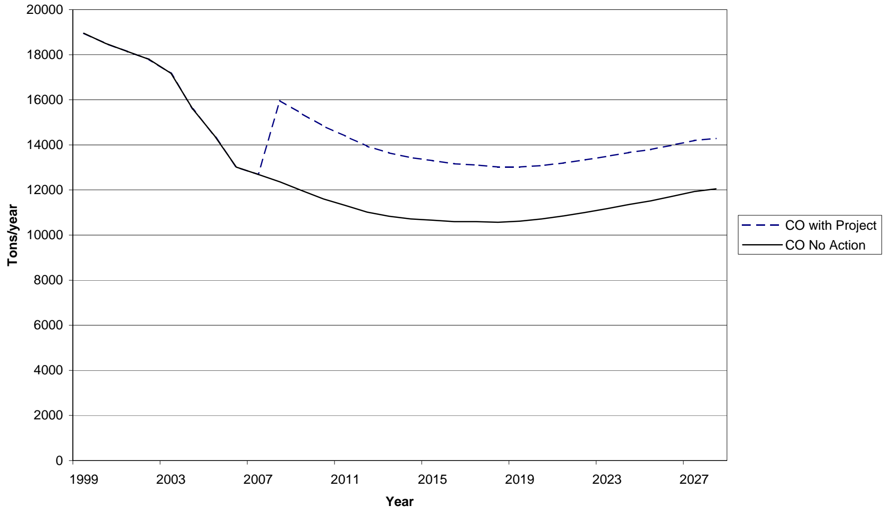
Figure K-2. Carbon Monoxide (CO) Emission Projections for Cascade Locks Resort and Casino and No Action Alternative
