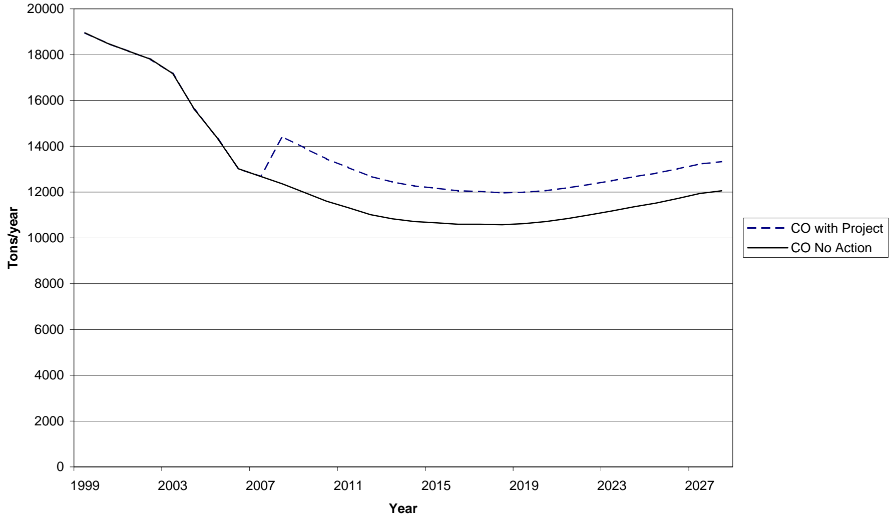
Figure K-7. Carbon Monoxide (CO) Emission Projections for Hood River Alternative and No Action Alternative
