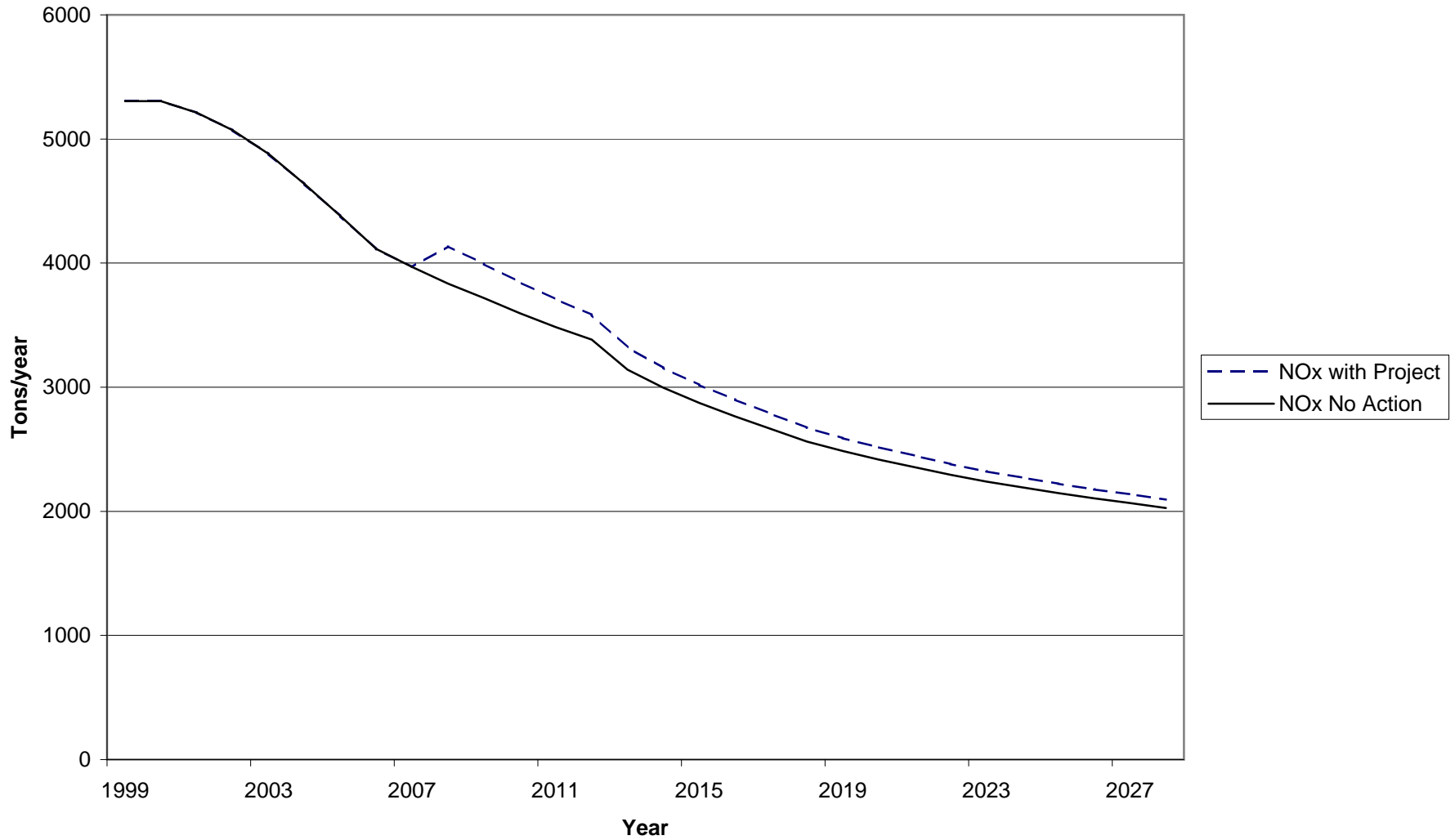
Figure K-9. Nitrogen Oxides (NO x ) Emission Projections for Hood River Alternative and No Action Alternative
