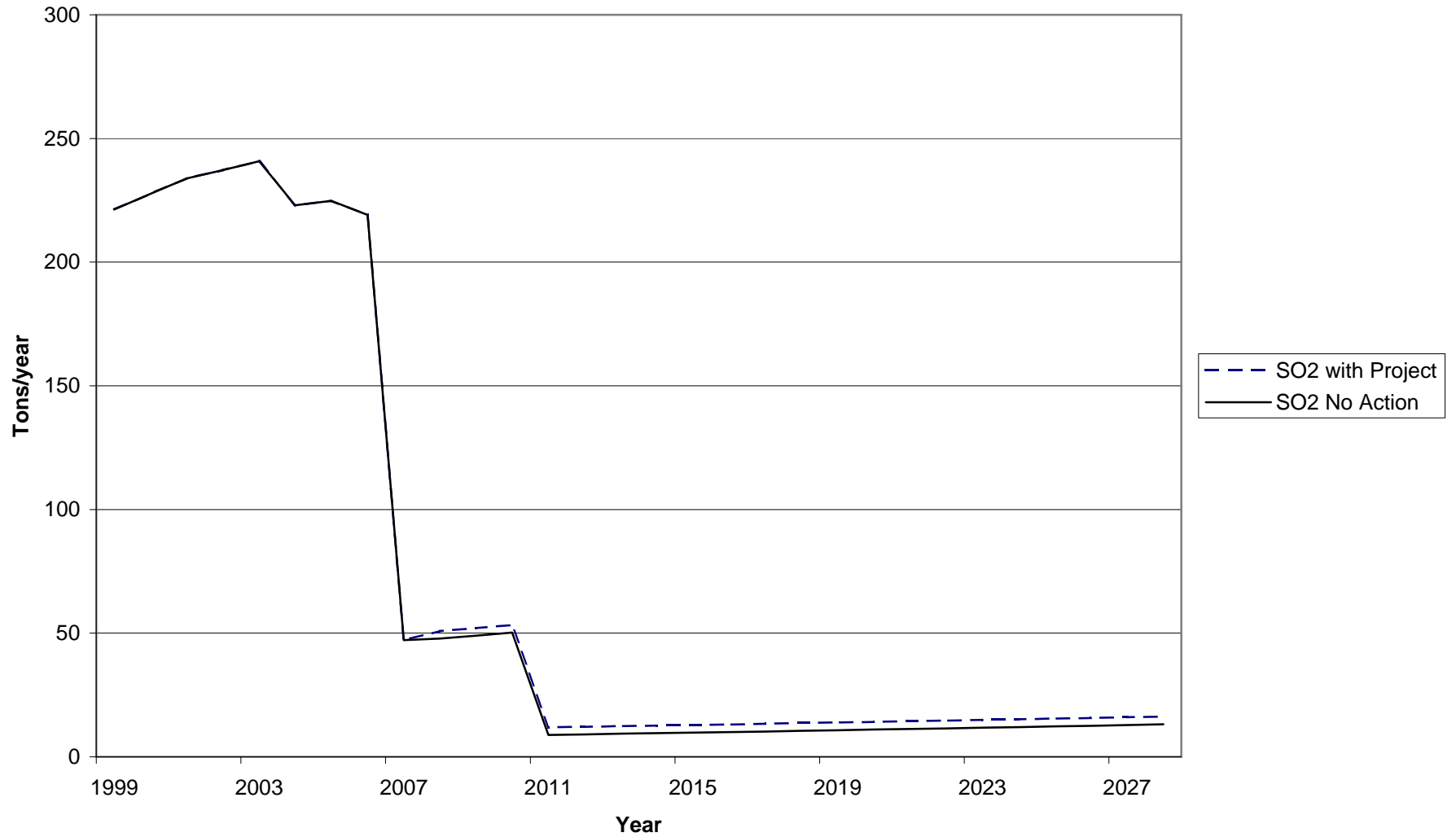
Figure K-10. Sulfur Dioxide (SO 2 ) Emission Projections for Hood River Alternative and No Action Alternative
