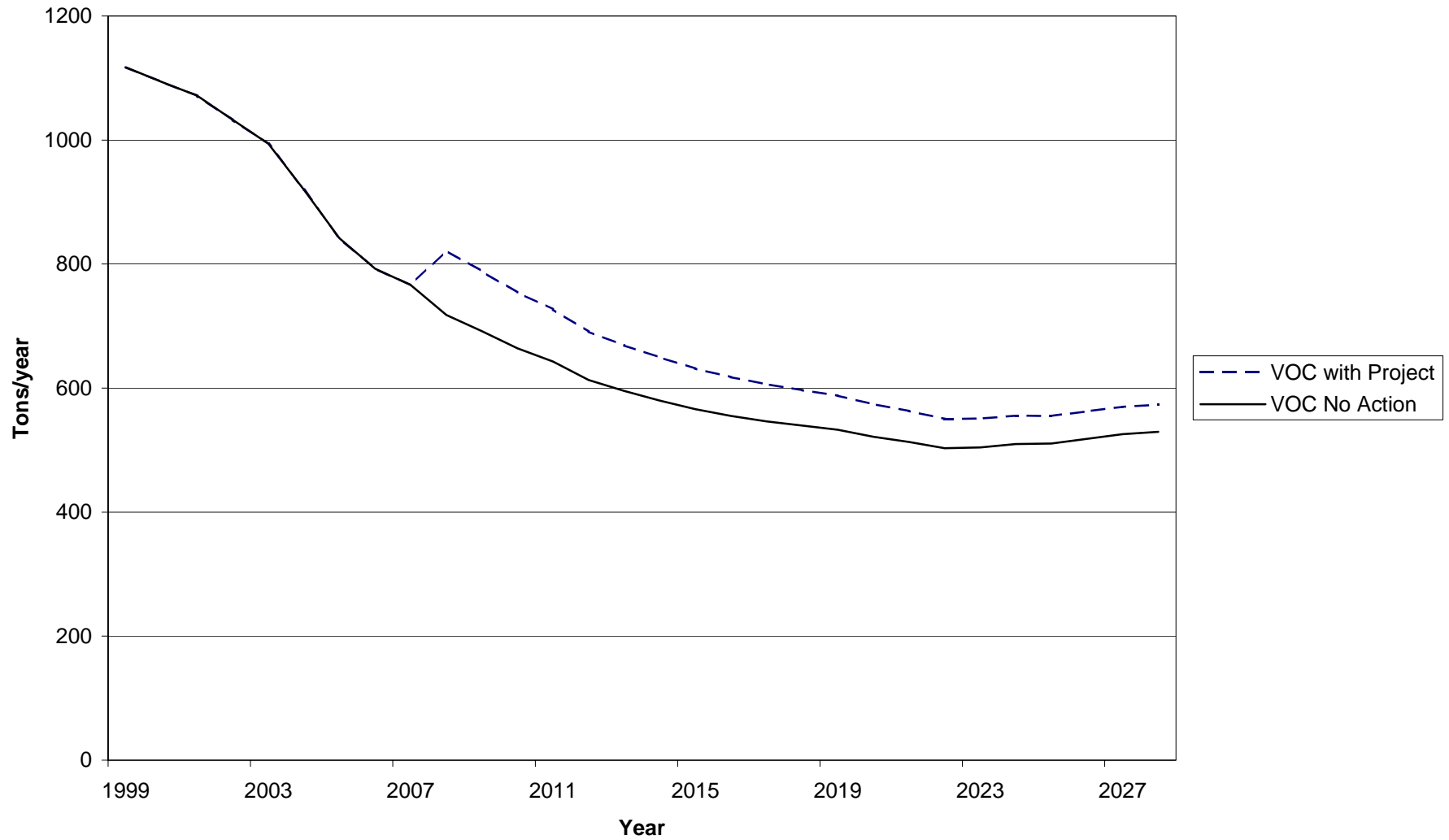
Figure K-6. Volatile Organic Compounds (VOC) Emission Projections for Hood River Alternative and No Action Alternative
