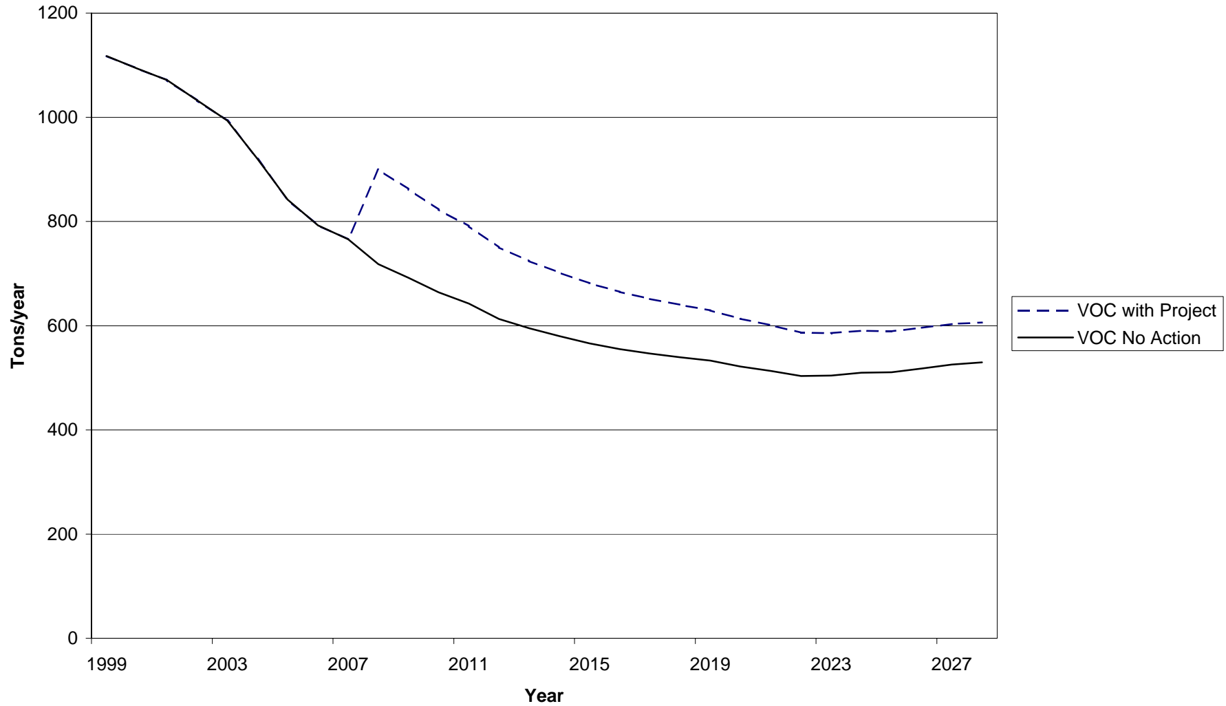
Figure K-1. Volatile Organic Compounds (VOC) Emission Projections for Cascade Locks Resort and Casino and No Action Alternative
