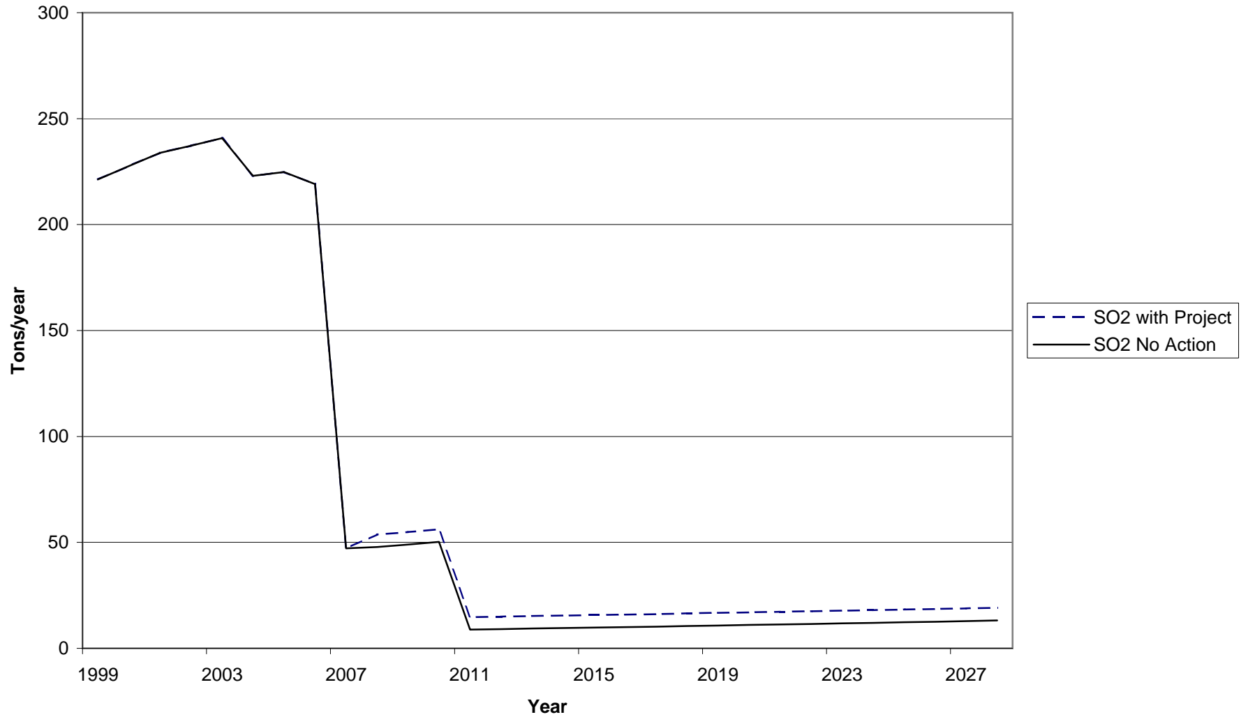
Figure K-5. Sulfur Dioxide (SO 2 ) Emission Projections for Cascade Locks Resort and Casino and No Action Alternative
