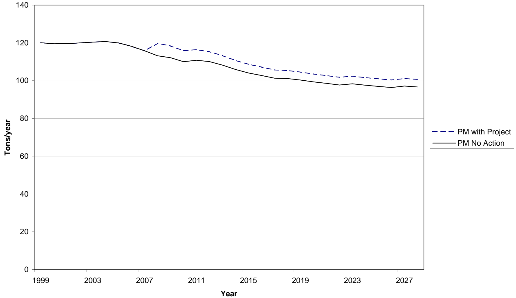
Figure K-8. Particulate Matter (PM) Emission Projections for Hood River Alternative and No Action Alternative
